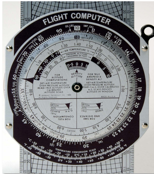
Reengineered Metal CSG (E6-B) Computer
